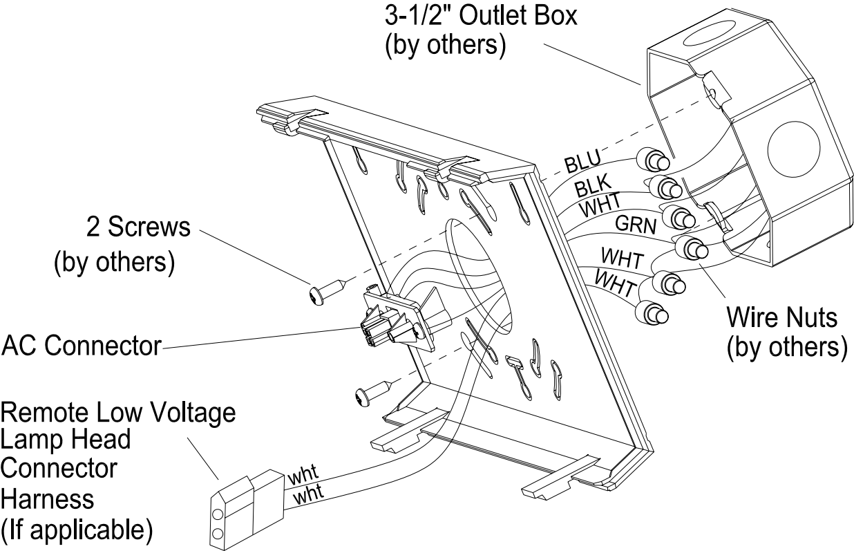
120VAC Hookup Shown Above
